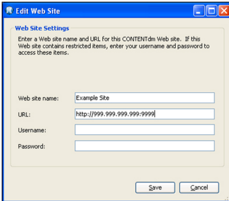
Figure 6: Editing Web site information.
